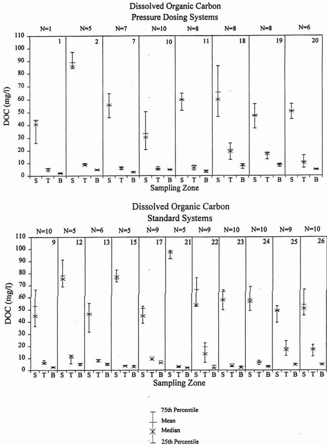
Figure 9. Dissolved organic carbon (DOC) concentrations for the septic tank (S), top zone (T) and bottom zone (B) for all systems. Sample number (N) and system number are shown at the top of each graph.
